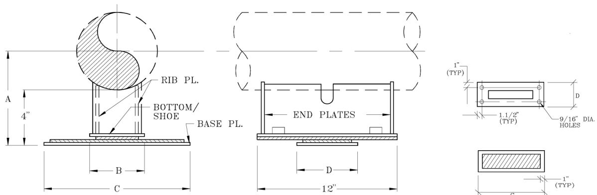
FIG. 501 - BOLTED BASE
