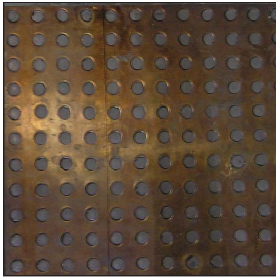
The Bronzphite and its cylindrical grooves filled with the graphite.
